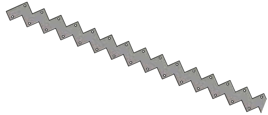
Code: E4959-B SHEET METAL ANGLE 45° COVER FOR FSN-401 / SUN LIGHT 20 mm / LEFT ALIGNMENT
